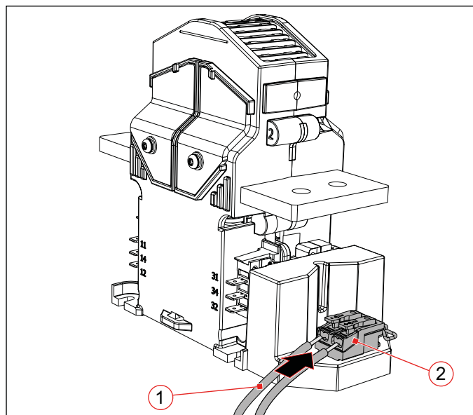
Fig. 11: C320K: Connecting the coil
