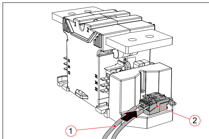
Fig. 12: C320S: Connecting the coil
