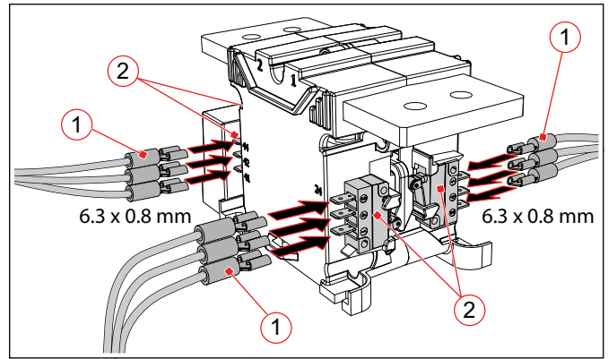
Fig. 10: C320S: Connecting the S870 auxiliary switches
